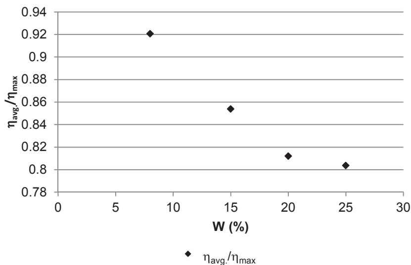
Figure 6. Influence of wood pellet moisture content on relative changes in \eta_{avg.}/\eta_{max} .
