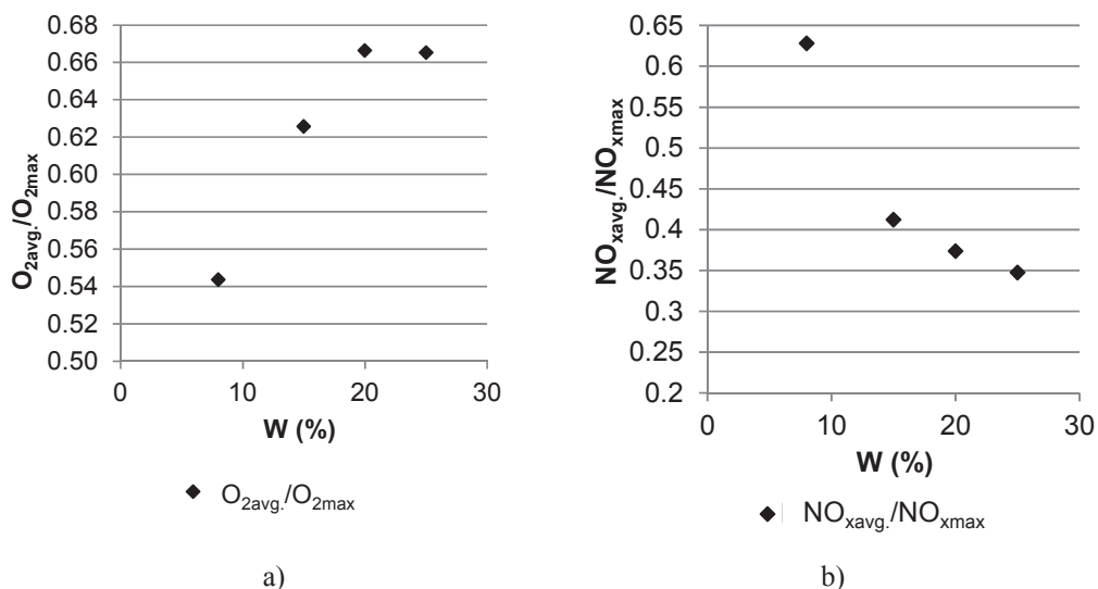
Figure 5. The influence of wood pellet moisture content on relative changes in O_{2avg.}/O_{2max} (a) and NO_{xavg.}/NO_{xmax} (b).
