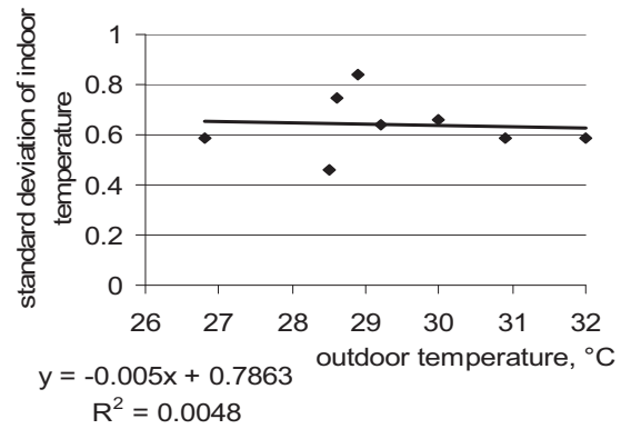
Fig. 3. Dependence of standard deviation of indoor temperature on outdoor air temperature.
