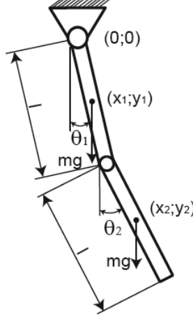
Figure 1. A physical double pendulum.
