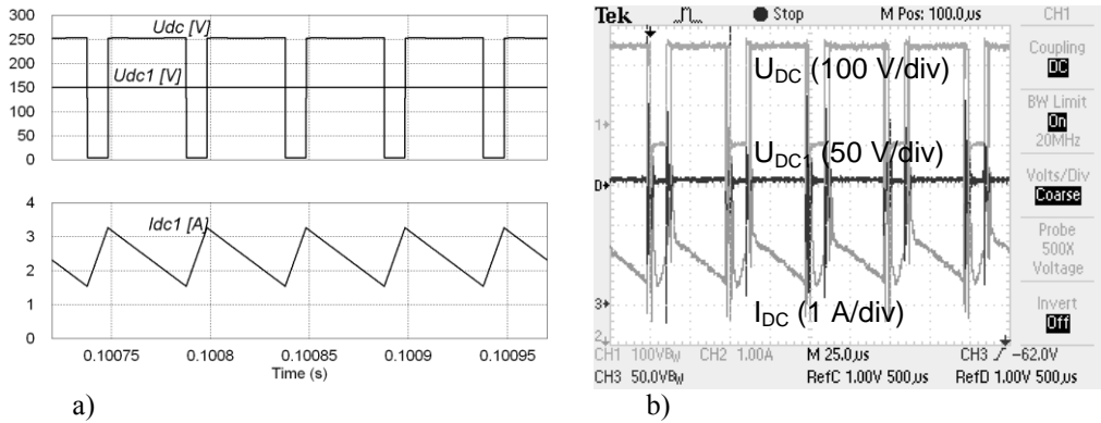
Figure 14. Simulated (a) and experimental (b) waveforms of generator side and intermediate DC link voltages and input current of the qZS based step-up DC/DC converter at 350 W.
