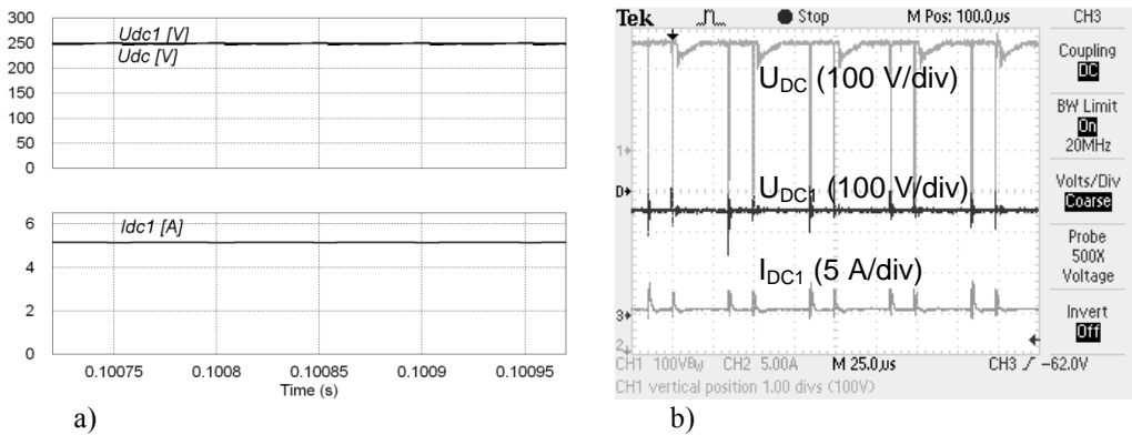
Figure 15. Simulated (a) and experimental (b) waveforms of generator side and intermediate DC link voltages and input current of the qZS based step-up DC/DC converter at 1,250 W.
