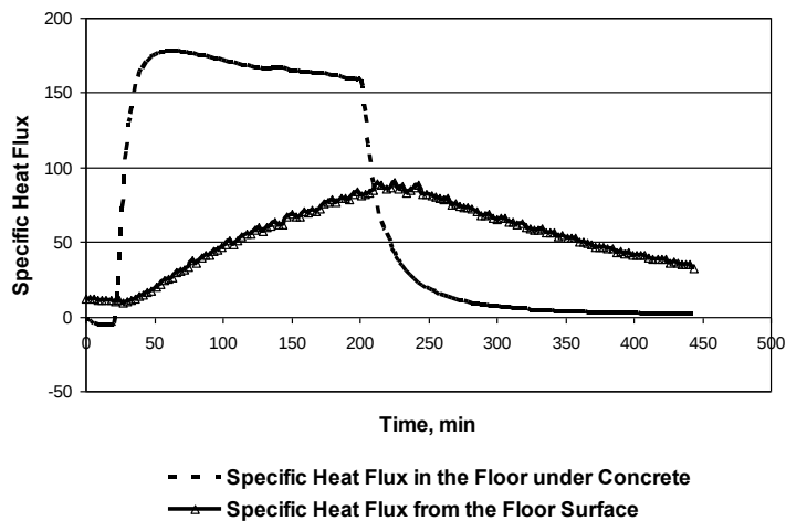
Figure 4. The specific heat flux ( \text{W m}^{-2} ) in the floor and from the surface to the air.
