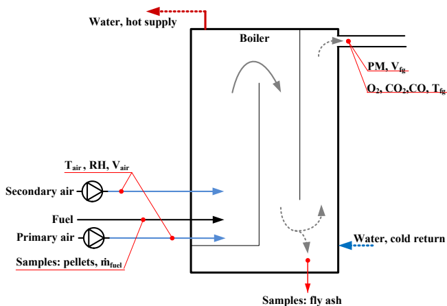
Figure 1. On-site pellet boiler and experimental system.
