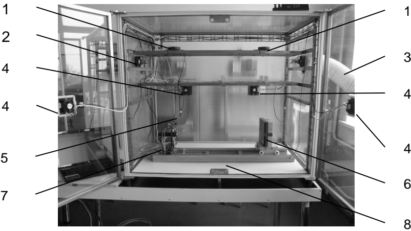
Figure 2. Microclimate chamber for simulation of greenhouse temperature and relative humidity: 1 – air recirculation fans; 2 – ventilation intake fan; 3 – ventilation outtake fan and tube; 4 – heating elements; 5 – temperature and humidity sensors; 6 – moving platform with target (container with water); 7 – sensor plate; 8 – rail for target moving.
