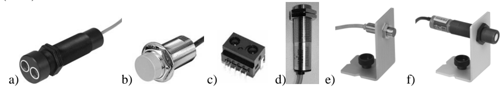
Figure 1. Experimental proximity sensors: a) – 170710; b) – CR30-15DN; c) –GP2Y0D340K; d) – 165342; e) – 177464; f) – 184118.
