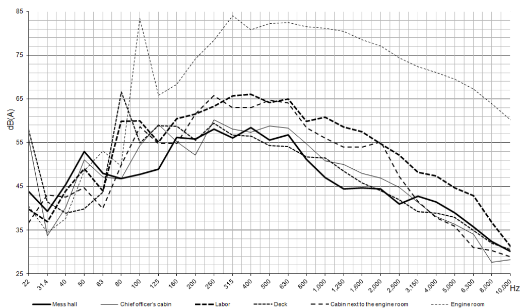
Figure 4. Ship, while anchored, noise frequency analysis.
