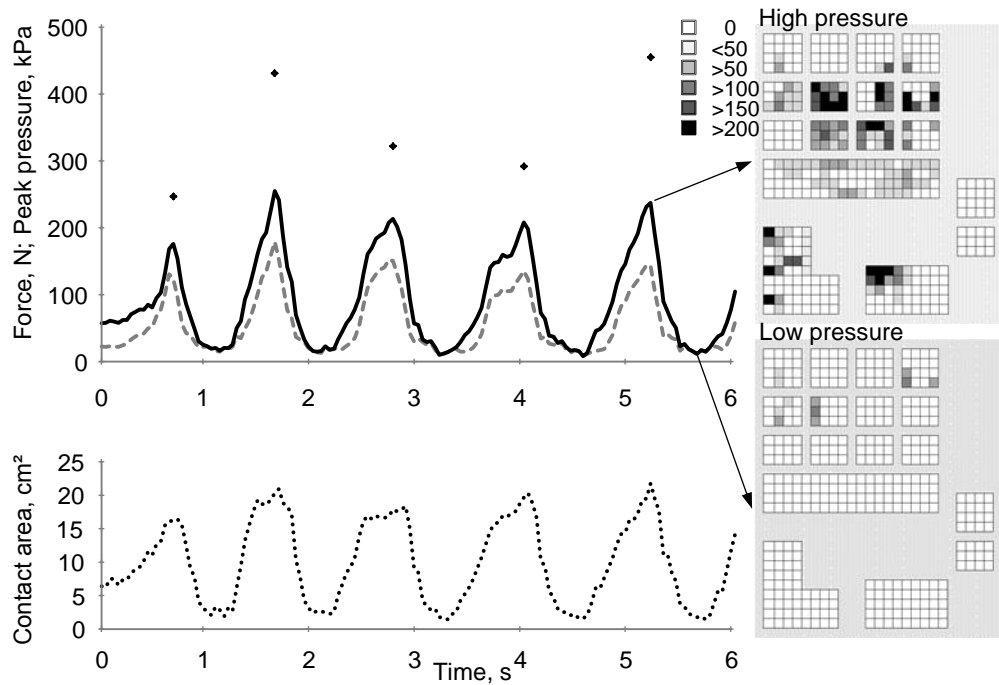
Figure 1. Sample analysis: work cycles (truns) while operating a screwdriver: dots – peak pressure on hand; solid line – force applied by whole hand; dashed line – force applied by fingers; dotted line – contact area; on the right, two GUI outputs are shown (high and low pressure frames), note that sensor regions correspond to Fig. 2-B (Own source, unpublished data).
