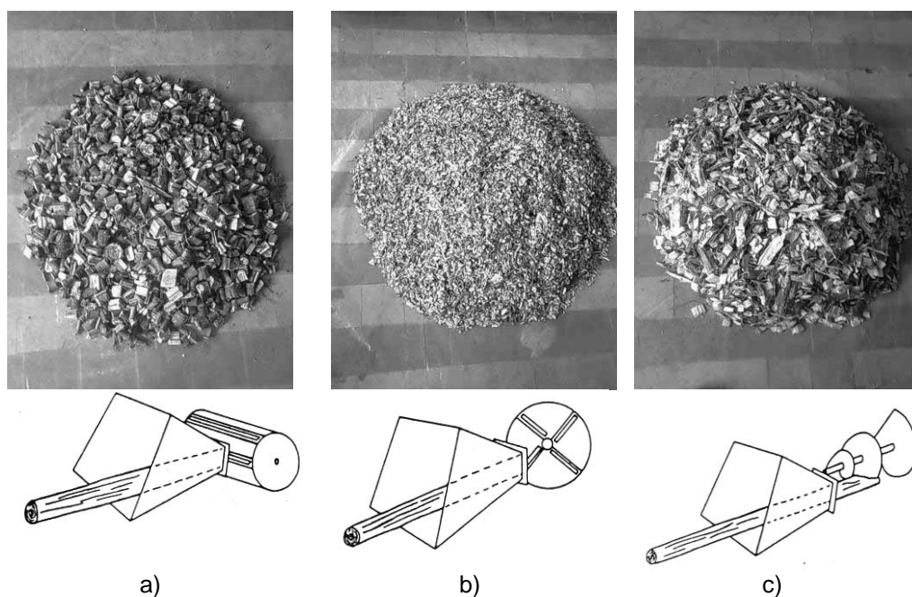
Figure 1. Various types of energy plant chopping mechanisms and the chaff quality: a) the drum chopper; b) the disc chopper; c) the screw chopper.
