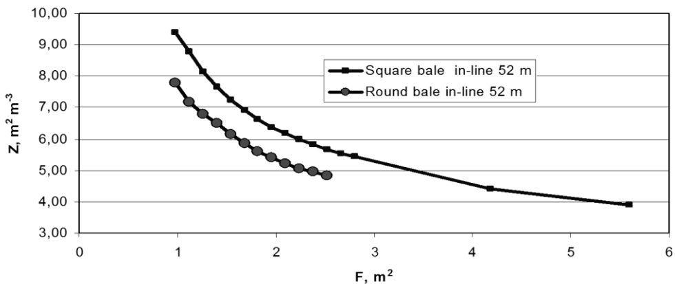
Figure 6. Impact of the cross-sectional area of the line bale F upon the consumption of the film Z ( L = 1.2 \text{ m} ; n = 50 ); for a round bale S_r = 0.25\pi D^2 ; for a line square bale S_{sq} = hL .
