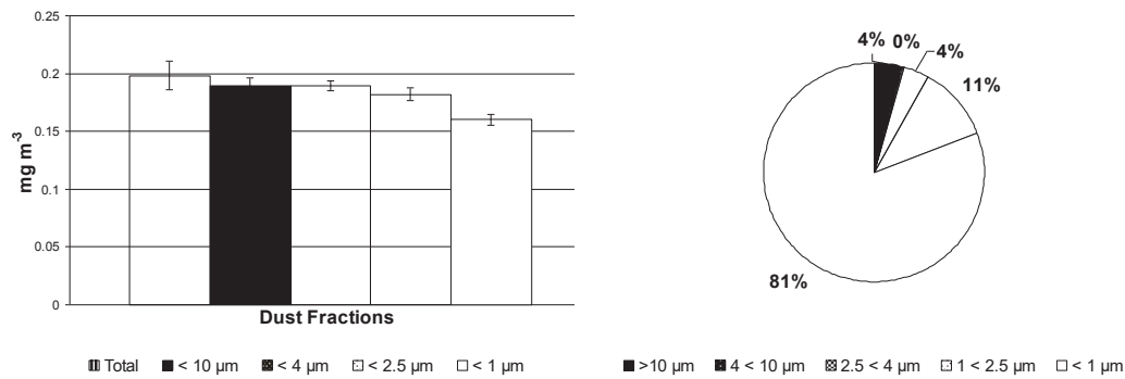
Figure 3. Concentrations and percentage of dust fractions inside the laboratory without ventilation.
