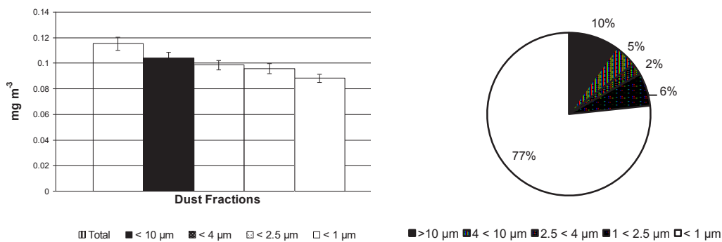
Figure 4. Concentrations and percentage of dust fractions inside the laboratory with ventilation level I.
