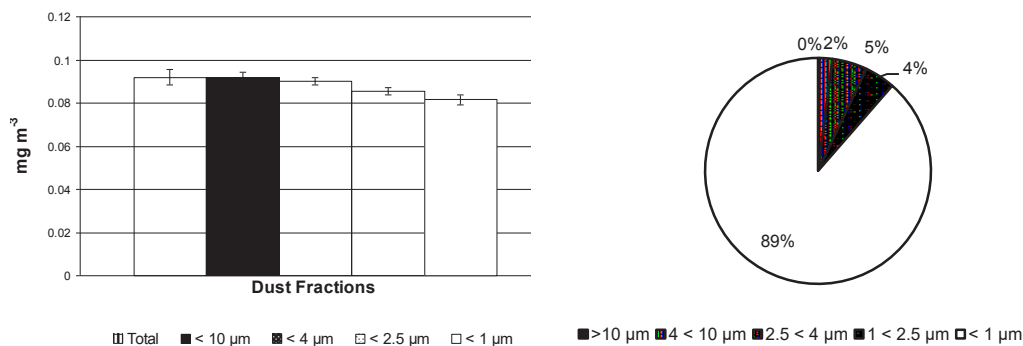
Figure 5. Concentrations and percentage of dust fractions inside the laboratory with ventilation level II.
