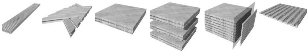
Figure 1. CWM production steps – starting from left to right hand (Dendrolight Latvija 2013).
