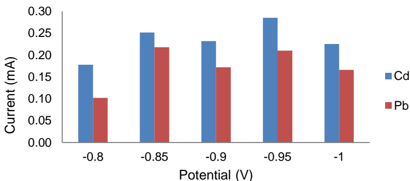
Figure 13. Accumulation potential anodic current peaks of 10 ppm of Cd 2+ and Pb 2+ from -0.80 V to -1.0 V.
