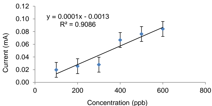
Figure 15. ASV Calibration curve for Cd 2+ using the optimized BiNP GPE electrode.
