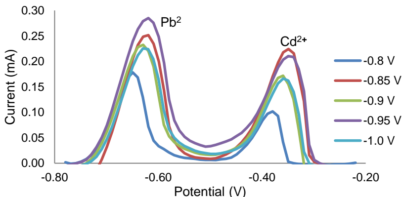
Figure 12. Anodic Stripping Voltammograms for the accumulation time of 10 ppm of Cd 2+ and Pb 2+ from -0.80 V to -1.0 V.
