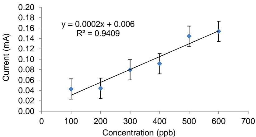
Figure 16. ASV Calibration curve for Pb 2+ using the optimized BiNP GPE electrode.
