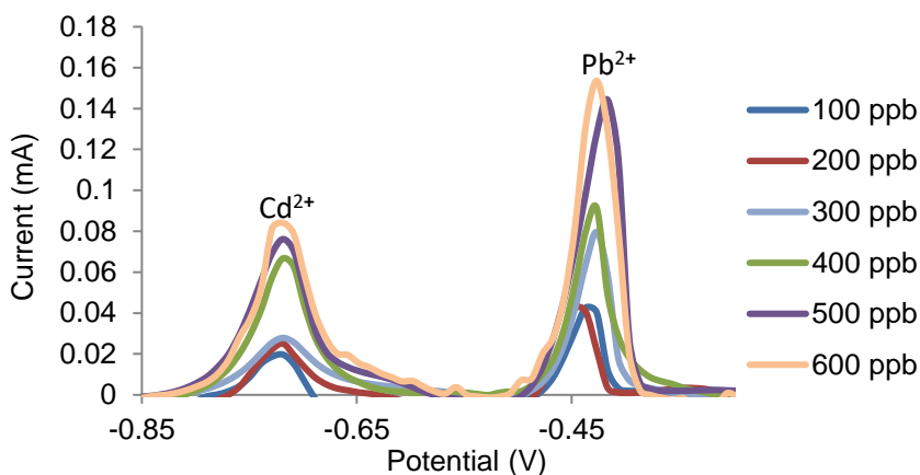
Figure 14. Anodic Stripping Voltammograms for various concentrations of Pb 2+ and Cd 2+ .
