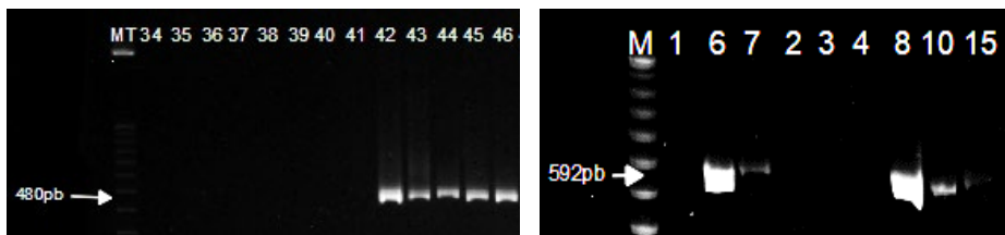
Figure 1. Electrophoretic profile of Botrytis spp. isolates, obtained by primers Bc108+/ Bc563- (left), CFM-NEP2/C-NEP2 (right).
