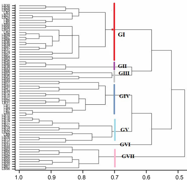
Figure 2. Dendrogram of Botrytis spp. isolates from various geographic origins, constructed using UPGMA algorithm.
