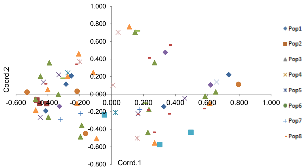
Figure 3. P CoA of Botrytis isolates using SSR primer data, classified by geographic origin.
