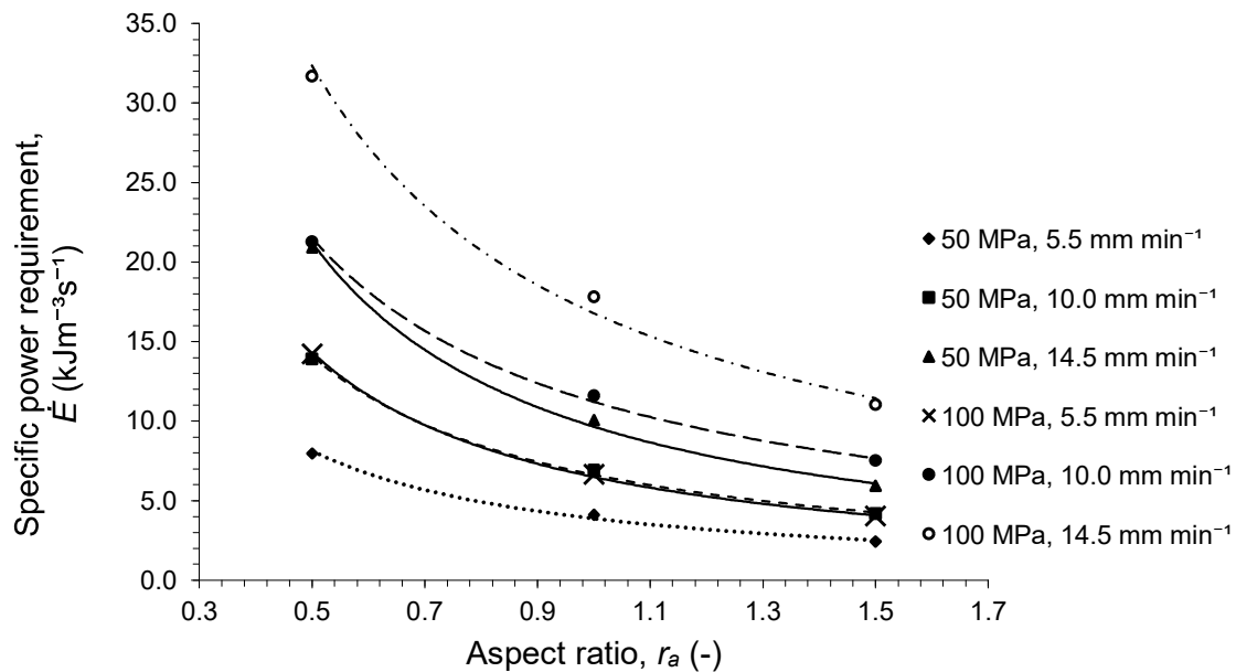
Figure 4. Specific power requirement as a function of the aspect ratio, 50 and 100 MPa of applied pressure and deformation rates of 5.5, 10.0 and 14.5 \text{mm min}^{-1} .
