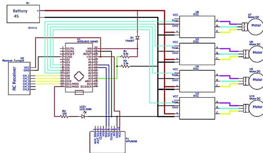
Figure 1. Electronic circuit diagram.
