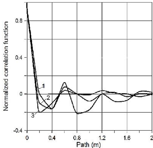
Figure 7. Normalized correlation functions of tillage depth oscillations at different operating speeds of combined tractor and harrow unit: 1) 2.1 m s -1 ; 2) 2.5 m s -1 ; 3) 3.3 m s -1 .
