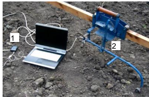
Figure 4. Device for measuring field profile oscillations: 1 – Arduino Uno; 2 – profilometer.
