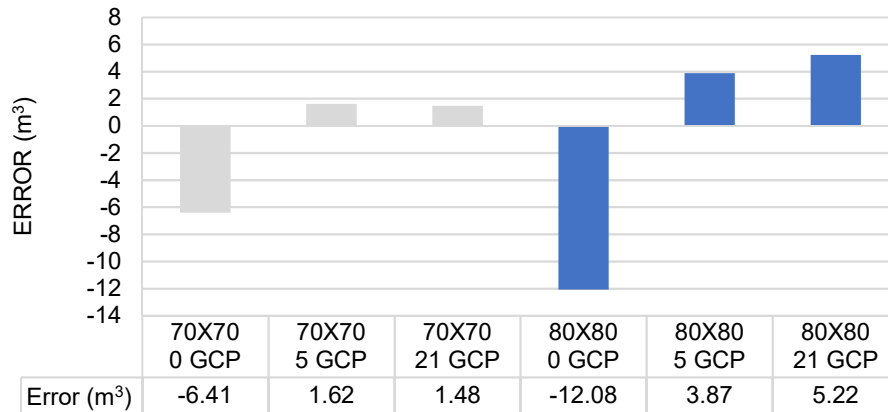
Figure 9. Absolute error ( \text{m}^3 ) between models generated from a covered composting pile and a model generated from laser scanning data.
