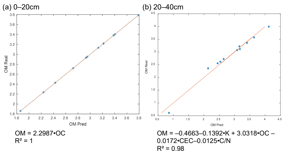
Figure 9. (a) soil organic matter as a function of organic carbon R^2 = 1 ; (b) organic matter as a function of exchangeable potassium, cation exchange capacity and C/N ratio. R^2 = 0.98 .
