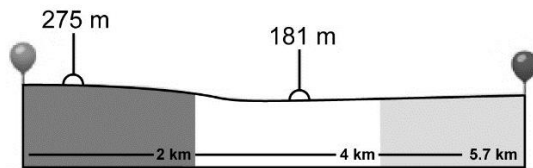
Figure 2. Line 107 road profile.
