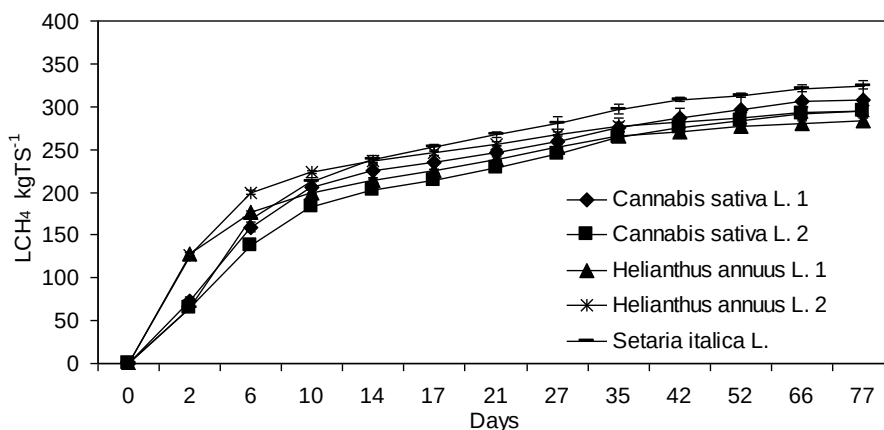
Figure 2. Accumulated methane production ( \text{LCH}_4 \text{ kgTS}^{-1} ) during 77 days of incubation at mesophilic temperature for perennial energy crops.
