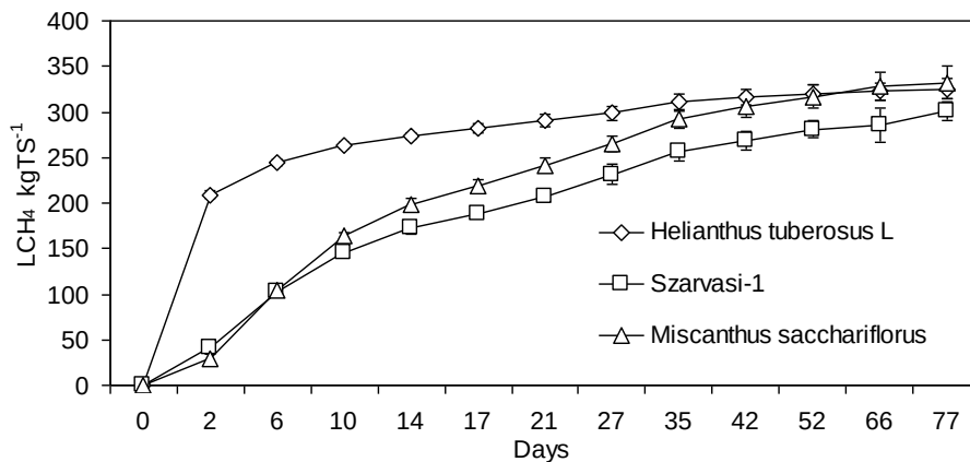
Figure 1. Accumulated methane production ( \text{LCH}_4 \text{ kgTS}^{-1} ) during 77 days of incubation at mesophilic temperature for perennial energy crops.
