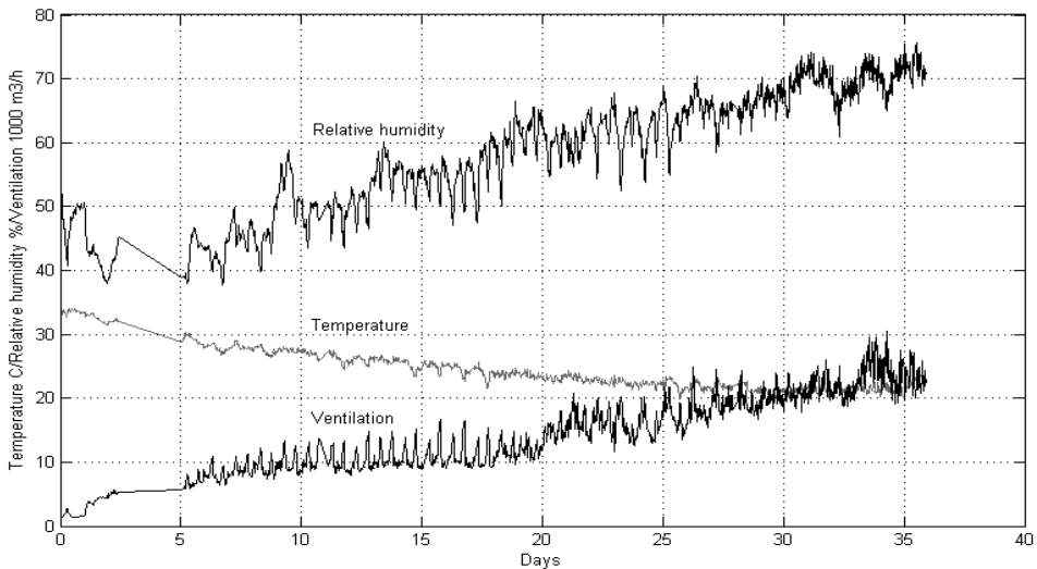
Fig. 2. Conditions inside the broiler house during one batch.
