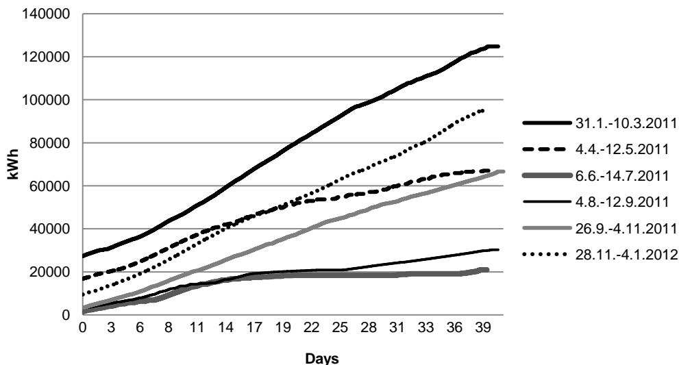
Fig. 4. Cumulated heating energy consumption during the six broiler batches.
