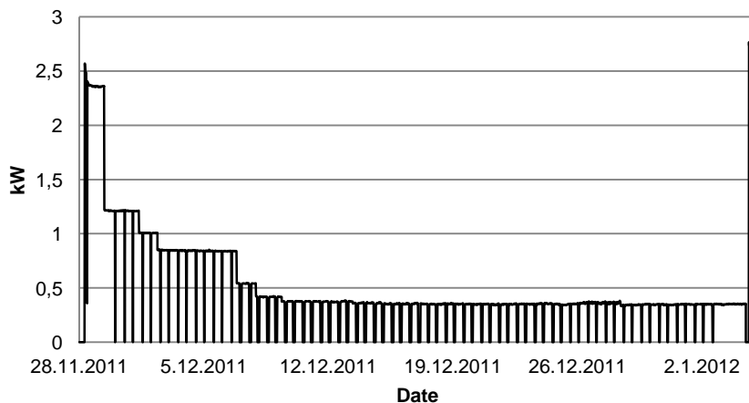
Fig. 6. Electricity power of lights during the one broiler batch.
