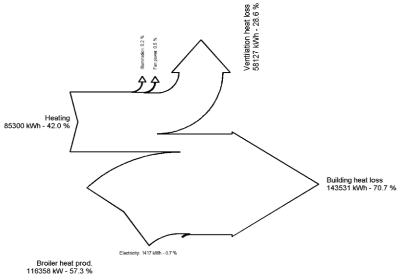
Fig. 3. Heat flows in broiler house.
