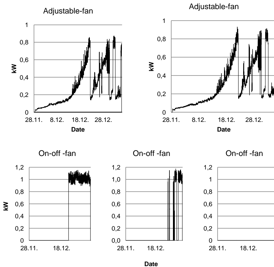
Fig. 5. Electricity power of on-off and adjustable -fans (median, n 6) during the one broiler batch.
