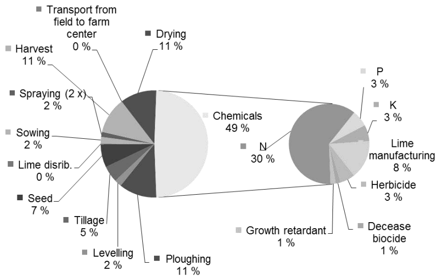
Figure 2. Energy consumption in barley production (14 GJ ha -1 ).
