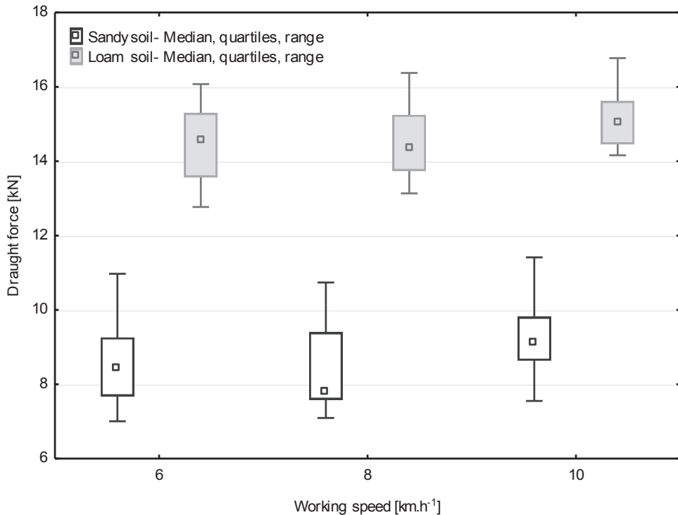
Figure 5. Dependence of draught force on working speed for sandy and loamy soil – working depth 0.15 m.
