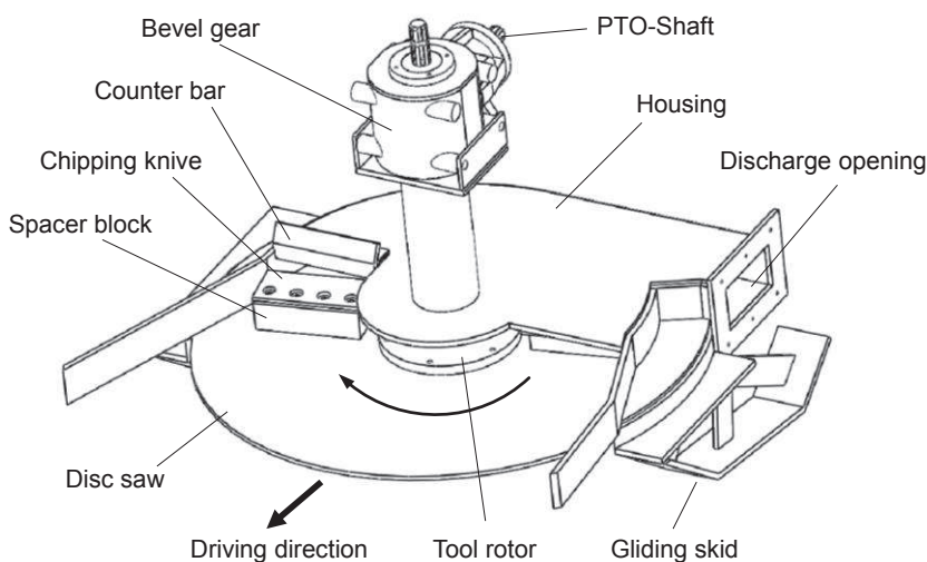
Figure 2. Principle of the ATB mower-chipper unit.
