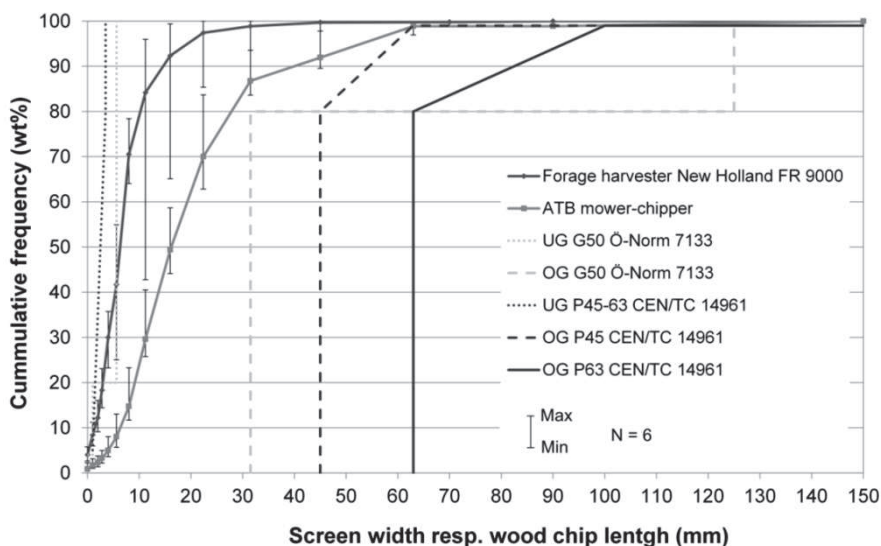
Figure 6. Particle size distributions of wood chips from poplar produced with different harvesters in 2013: Forage harvester New Holland FR 9000 ... fine chips P 45/G30; ATB tractor-mounted mower-chipper ... coarse chips P 45/G50.
