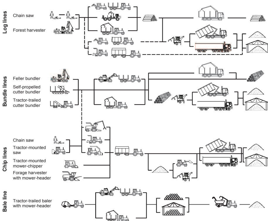
Figure 1. Systematics of harvest and post-harvest technologies for short rotation coppices.
