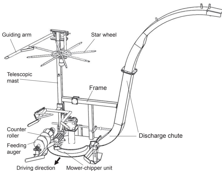
Figure 3. Principle of the ATB mower-chipper unit.
