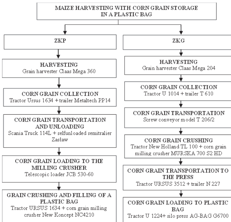
Figure 1. Scheme of the technology for corn grain ensiling in a plastic bag.
