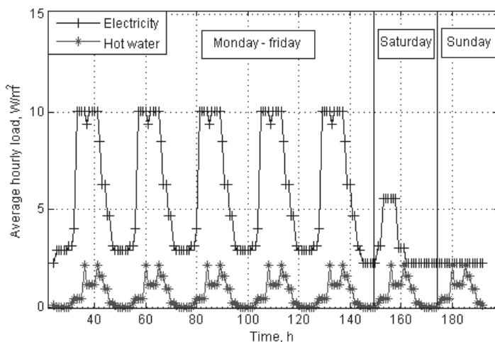
Figure 2. Hot water and electricity consumption load profiles for a typical weekday and weekend.
