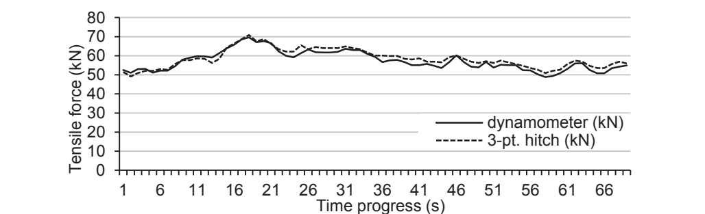
Figure 4. Time record of tensile forces measured with a tractor’s in-built sensor and the dynamometer LUKAS type S-38 on field No. 2.
