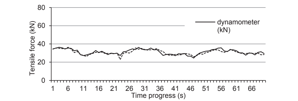
Figure 3. Time record of tensile forces measured with a tractor’s in-built sensor and the dynamometer LUKAS type S-38 on plot No. 1.
