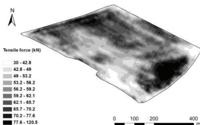
Figure 5. Map of the tensile force measured with a John Deere 8320 tractor.
