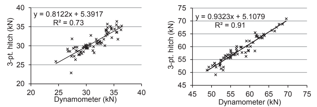
Figure 2. The dependence of the tensile force of a 3-pt. hitch on the values received from the dynamometer LUKAS type S-38 measured on field No. 1 (left side) and field No. 2 (right side).
