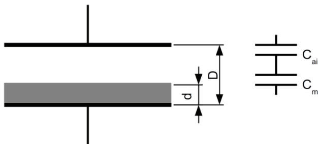
Figure 1. The diagram of the capacitive throughput sensor: D – the distance between electrodes; d – the thickness of the material layer, C_{air} ; C_m – the capacitance of the substituted capacitors.
