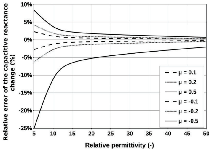
Figure 3. The relationship between the relative error of the capacitive reactance change and the relative permittivity of the measured material.
