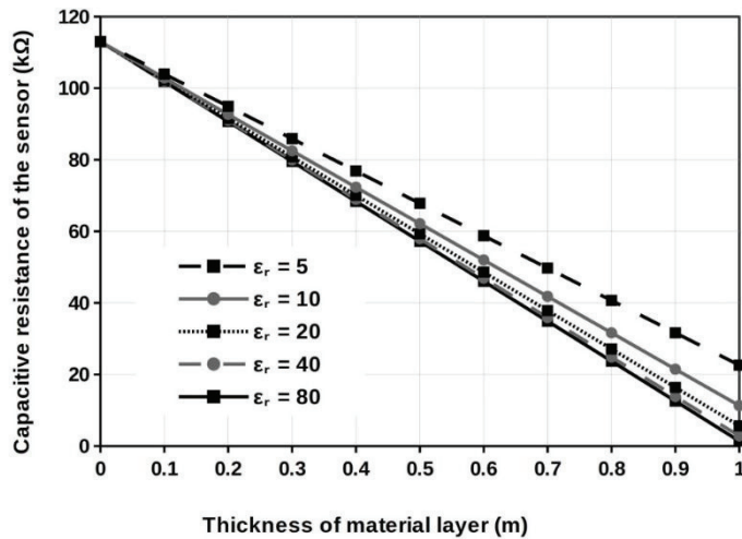
Figure 2. The dependence between the capacitive reactance of the sensor and the material thickness layer.
