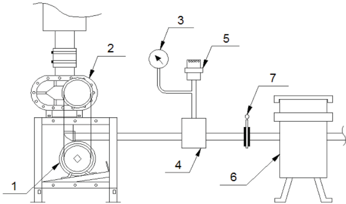
Figure 3. Diagram of the measurement of the performance of the vacuum pump: 1 – motor; 2 – vacuum pump; 3 – vacuum gauge; 4 – valve; 5 – flow meter; 6 – filter; 7 – slide.
