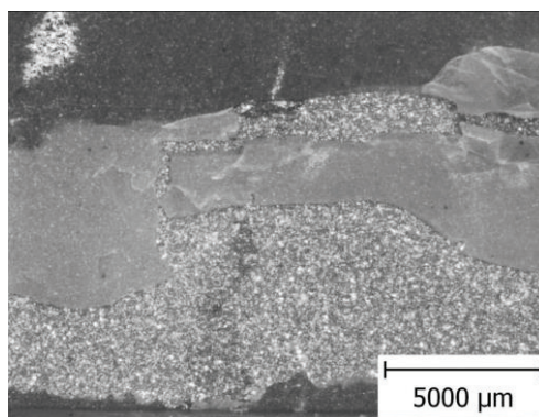
Figure 5. Adhesive-cohesive failure area – adhesive contaminated with dusty particles of size 315 μm and concentration 1,000 mg.
