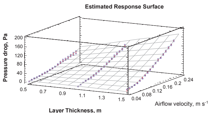
Figure 5. Estimated response surface for pressure drop.
