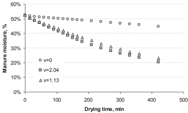
Figure 8. Changes of the manure moisture at tray with holes size 4 mm and with different forced air speeds v ( \text{m s}^{-1} ).
