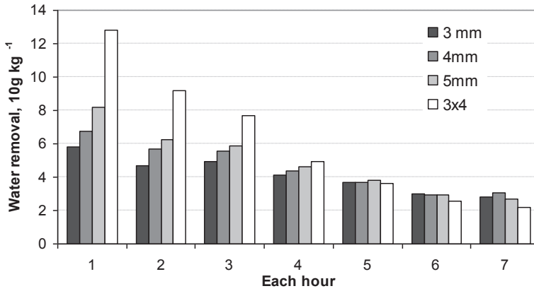
Figure 7. The moisture removal from the manure ( 10\text{g kg}^{-1} ) with initial manure moisture 52.4%, at each hour of drying with air speed at bottom 2.04\text{ m s}^{-1} .
