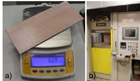
Figure 1. Adhesive spread control (a) and panel pressing (b).
