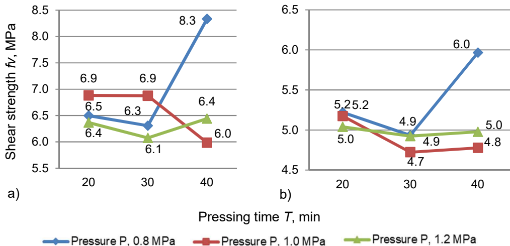
Figure 6. The influence of pressing time T and bonding pressure P interaction on the shear strength of: a – eucalyptus wood bonded with EPI-1 adhesive and b – radiata pine wood bonded with EPI-2 adhesive.
