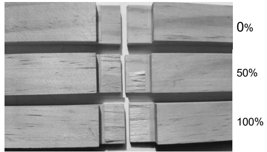
Figure 3. Wood failure percentage examples with wood failure 0%, 50% and 100%.
