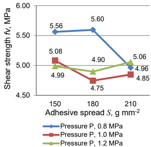
Figure 7. The influence of adhesive spread S and bonding pressure P interaction on shear strength of radiata pine wood bonded with EPI-2 adhesive.
