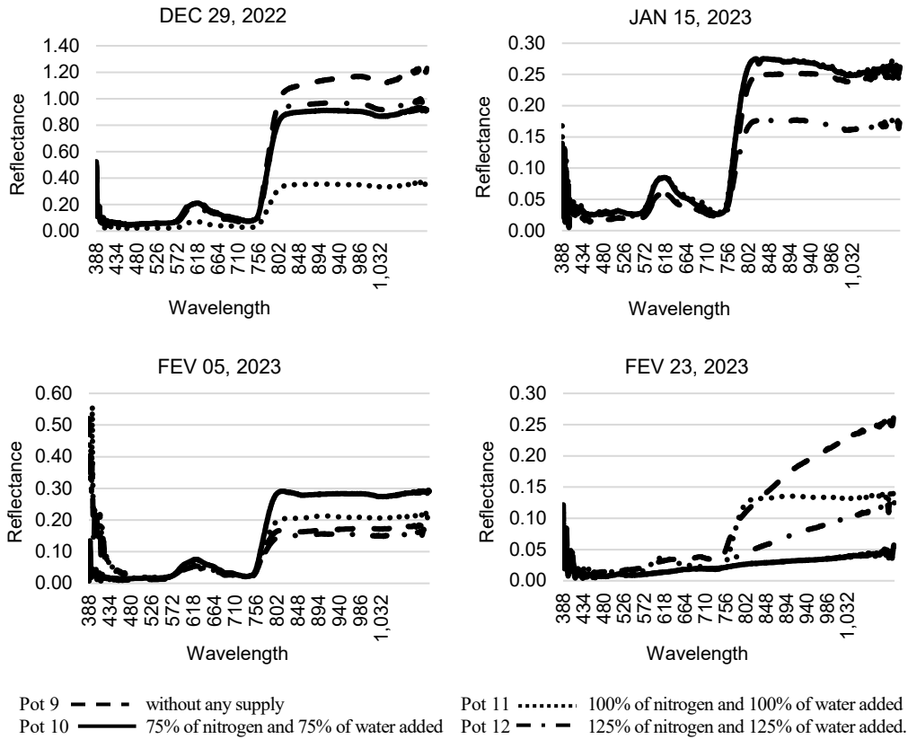
Figure 4. Evolution of mint reflectance with variable nitrogen and water supply (case N o 3).
